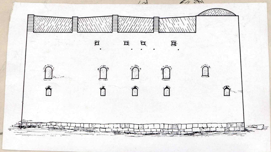
The Castle; restored elevation of west face
